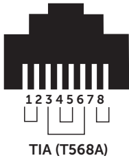
T568A Cabling Pinout Specifications
