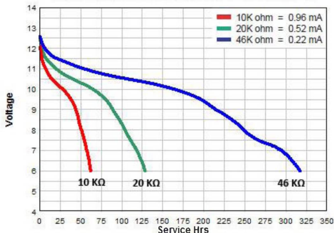
Continuous Discharge @ Room Temperature
